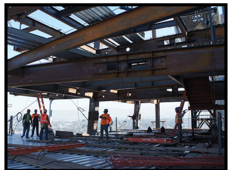
Structural Steel Erection
